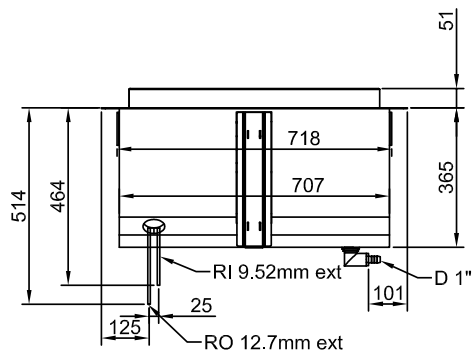
Rear side
